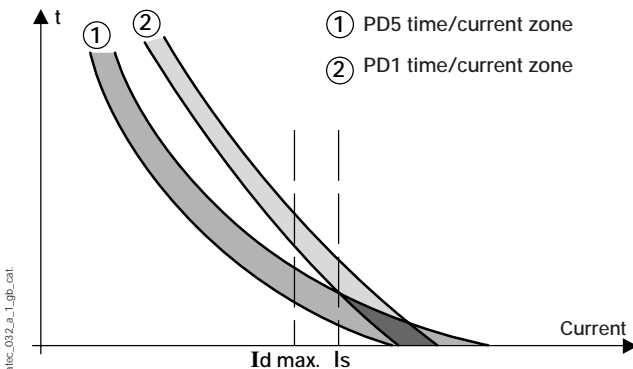
Fig. 3: partial discrimination
