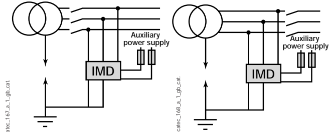
Fig. 3: IMD connection after the master switch
