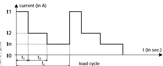
Fig. 4: cyclic overload
