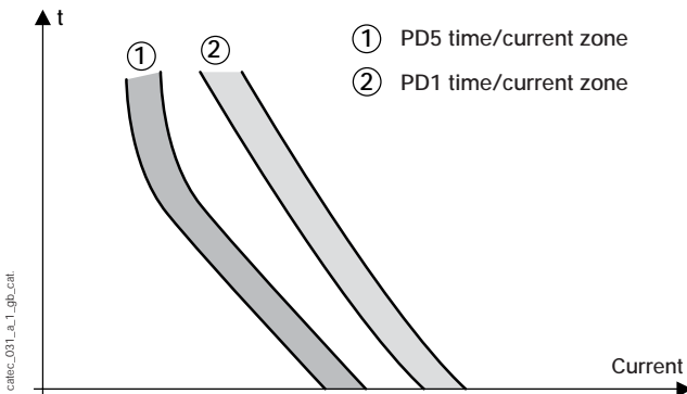
Fig. 2: total discrimination
