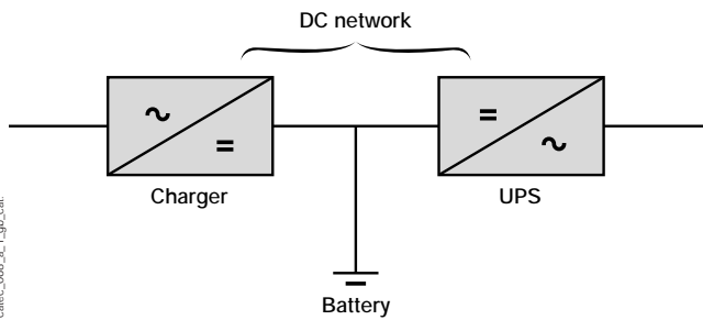
Fig. 3: IMD on network supplied by UPS
