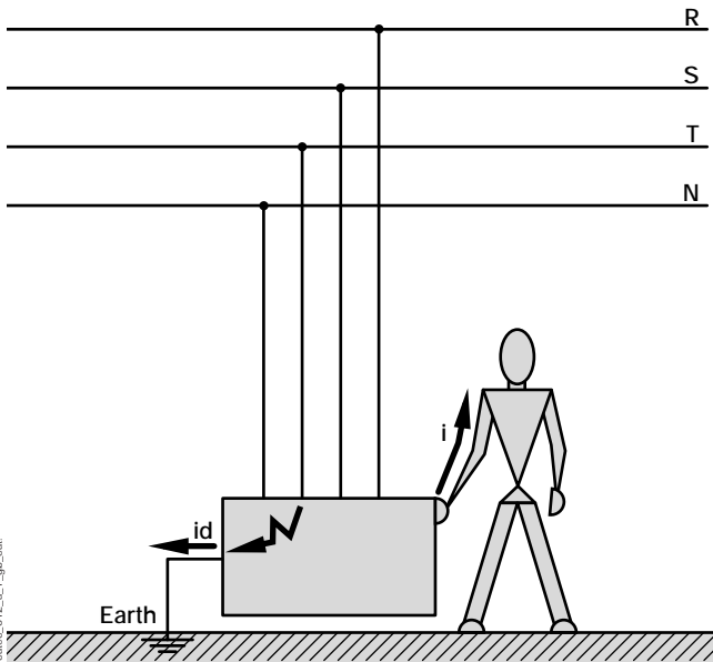
Fig. 1: indirect contact
