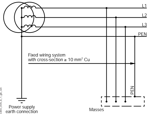
Fig. 2: TNC arrangement
