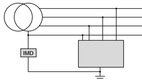
Fig. 2: IMD connection: inaccessible earth
