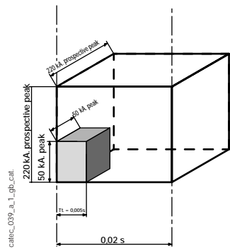
Fig. 4: limiting I 2 t 1 x 1 x t
