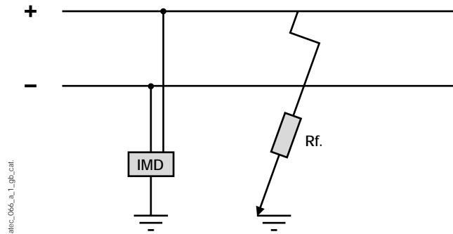
Fig. 1: asymmetrical fault
