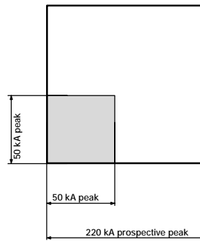
Fig. 3: limiting electrodynamic forces proportional to squared current
