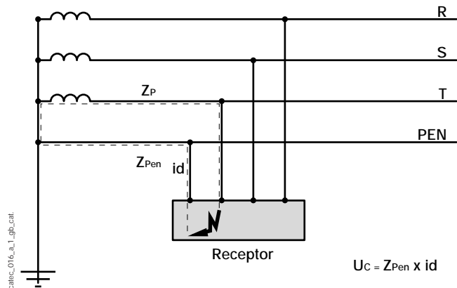
Fig. 2: TN load current fault
