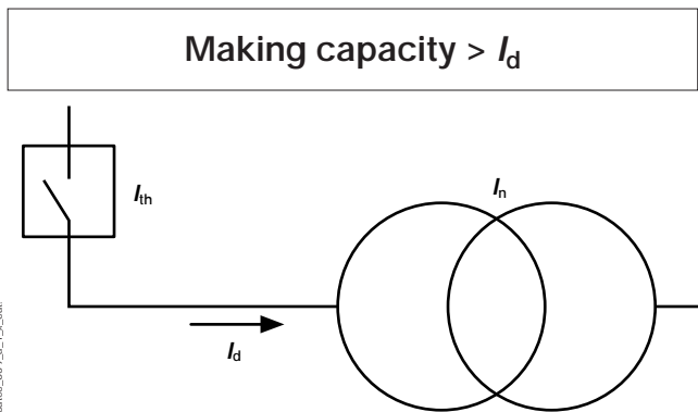
Fig. 2: switch at transformer primary
