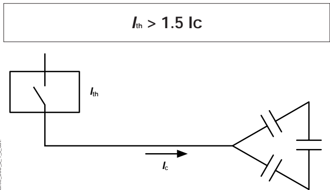
Fig. 1: switch upstream of capacitors
