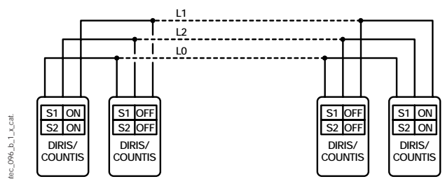
Fig. 3: example of DIRIS connection
