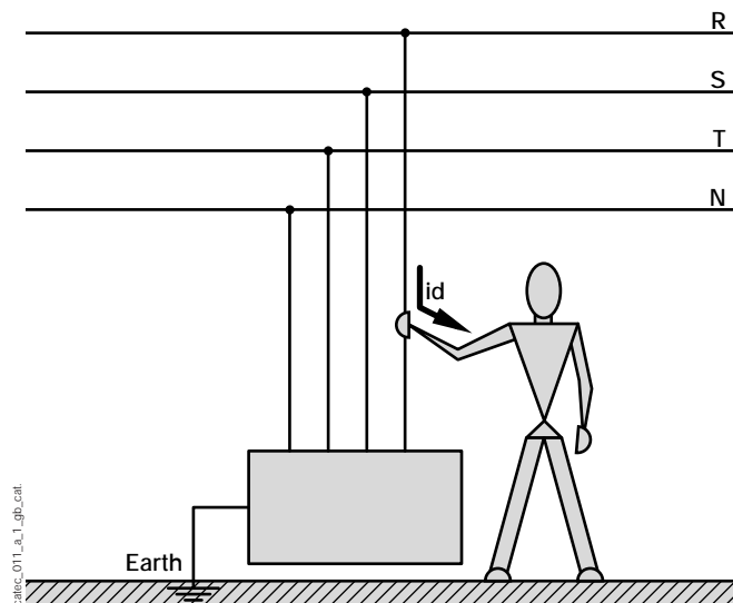
Fig. 1: direct contact
