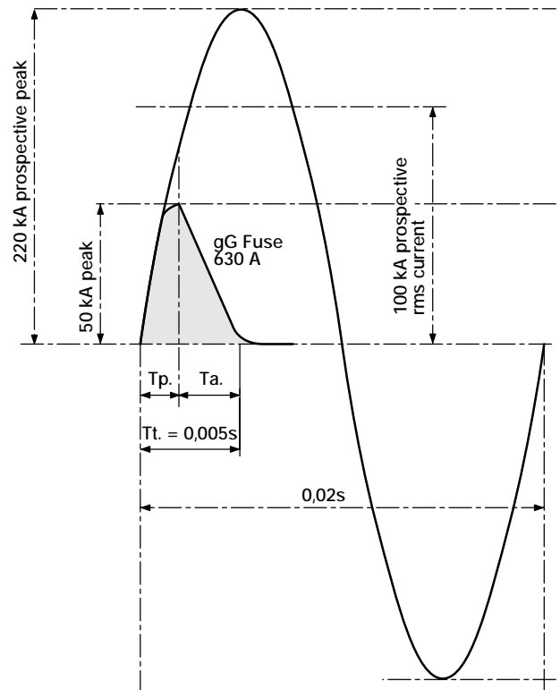
Fig. 2: cut-off peak current
