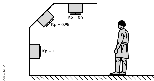
Fig. 2: position de-rating
