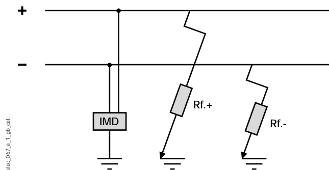
Fig. 2: symmetrical fault
