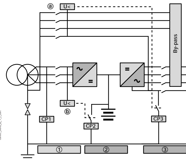
Fig. 1: monitoring insulation on control circuits
