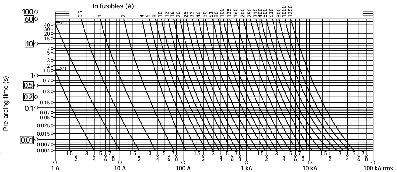
► Time/current characteristics (IEC standard)
