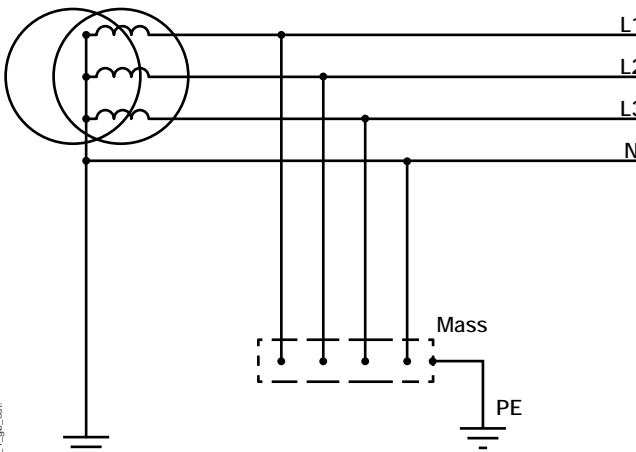
Fig. 1: TT arrangement
