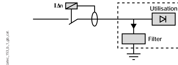
Fig. 1: connection of IMD: general case
