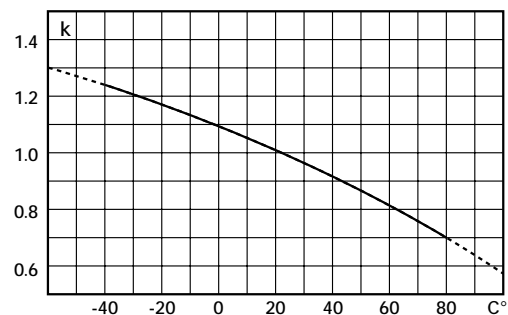
Fig. 2: K_{TUR} correction factor
