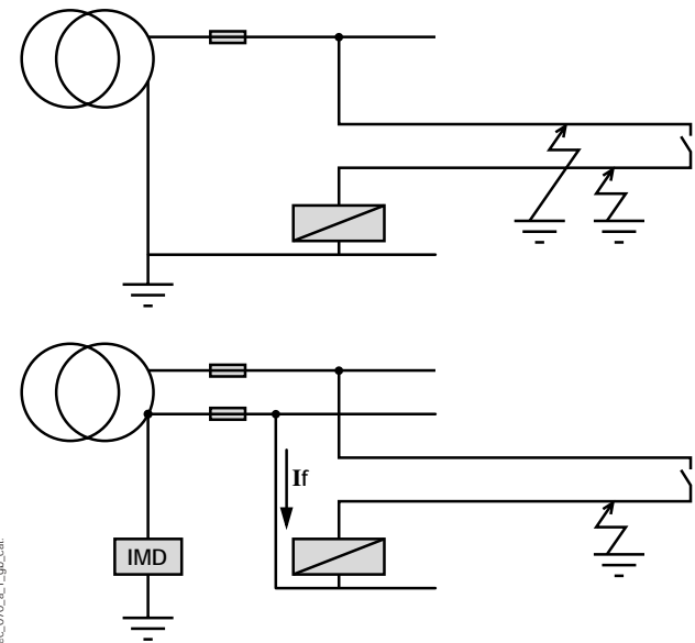
Fig. 1: monitoring insulation on control circuits
