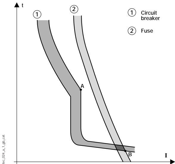
Fig. 1: fuse/circuit breaker discrimination
