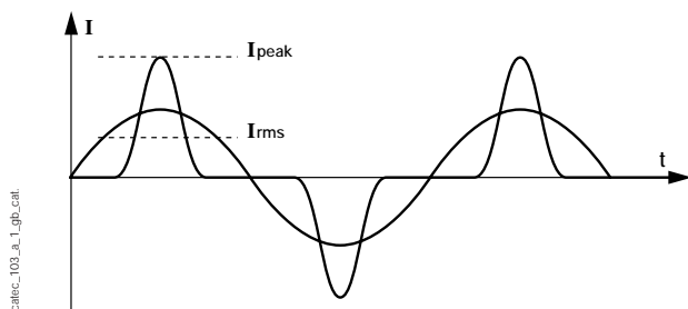
Fig. 6: peak factor: fp = I_{peak}/I_{rms}
