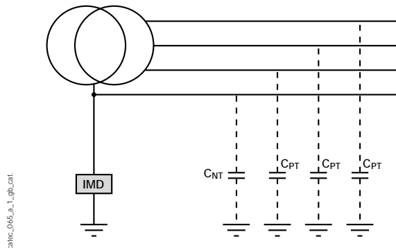
Fig. 2: earth leakage capacitance on an AC network
