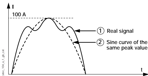
Fig. 1: measurement distortion
